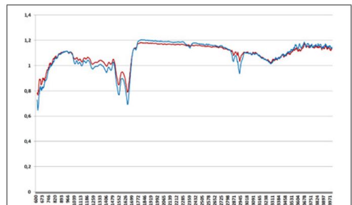
Figure 6: IR spectroscopy of the inner surface of the right elbow joint. spectrum of the right elbow joint area before treatment spectrum of the right elbow joint area after RayForce
