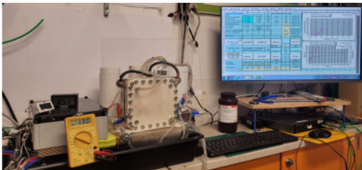
Figure 1: AEL 100 laboratory cell and PC-controlled experimental test station.
