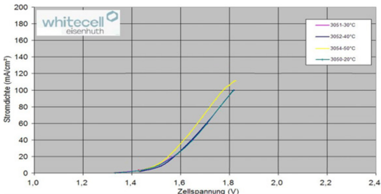
Figure 4: U-j characteristics of the optimized synthetic-seawater/KOH test series at different temperatures.
