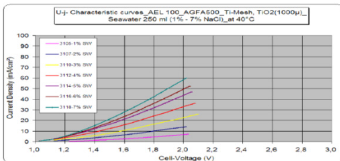
Figure 3: Influence of NaCl concentration between 1 and 7 wt.% on the current density at 40 °C.
