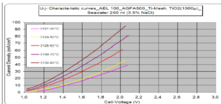
Figure 2: Effect of temperature on the U-j characteristics of the seawater cell operated with 3.5 wt.% NaCl.
