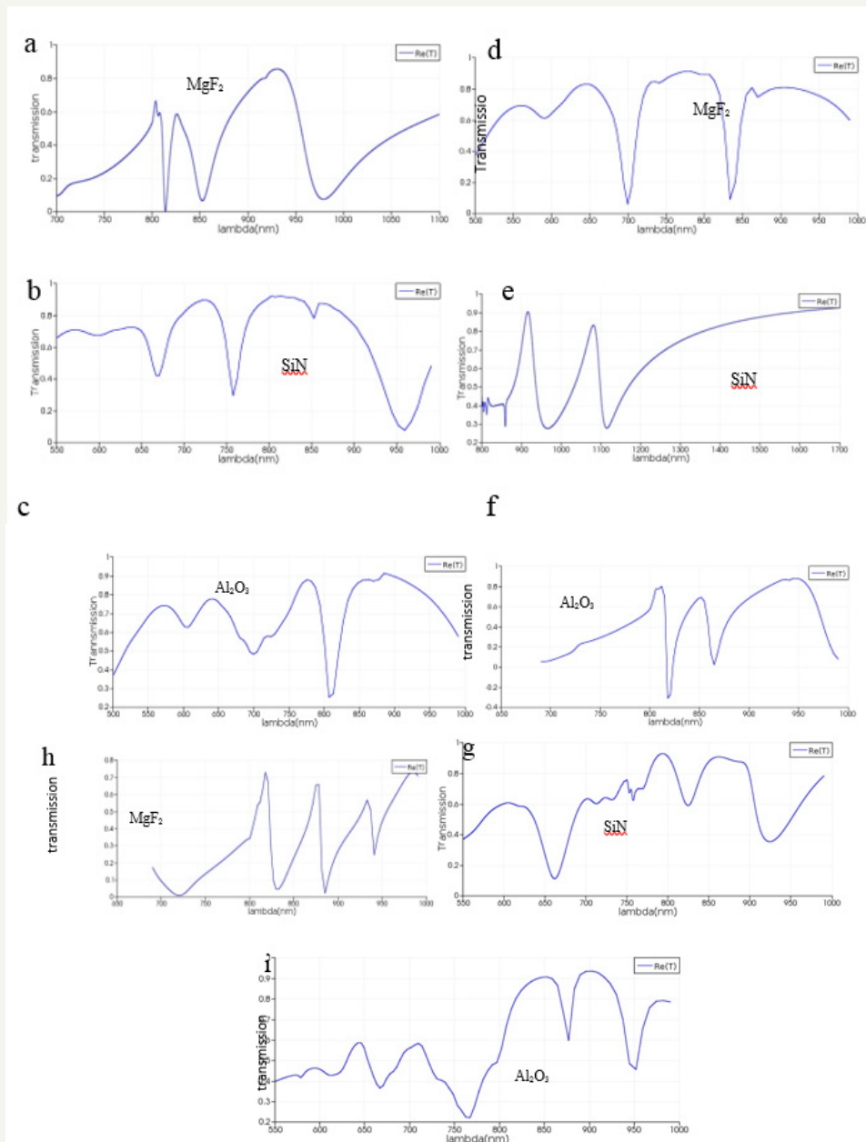
Figure 2: The transmission spectrum Vs wavelength with different refractive indices for the proposed models of plasmonic nano antennas: a, b and c for dual U, dual T. d, e and f for single U, dual L. g, h and i dual U, 4L.
