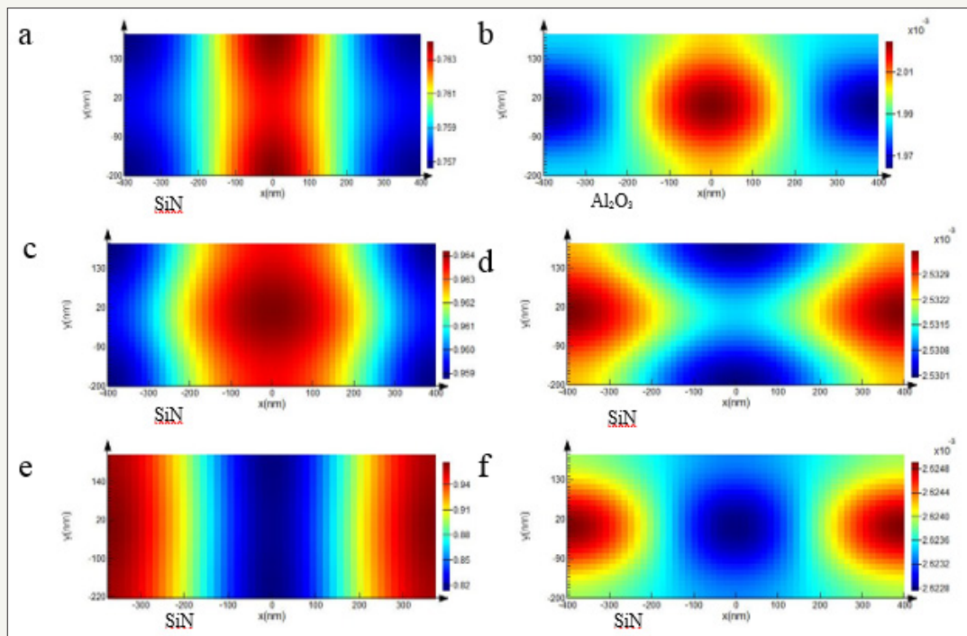
Figure 3: best field distributions of E and H; a and b represent E,H for dual U, dual T. c and d represent E,H for single U, dual L. e and f represent E,H for dual U, 4L.
