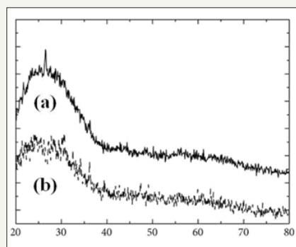
Figure 2: X-Ray Photoelectron Spectroscopy (XPS) analysis of malignant human cancer cells and tissues; 1a: before and 1b: after irradiating of synchrotron radiation in transformation process to benign human cancer cells and tissues with the passage of time [1–141].
