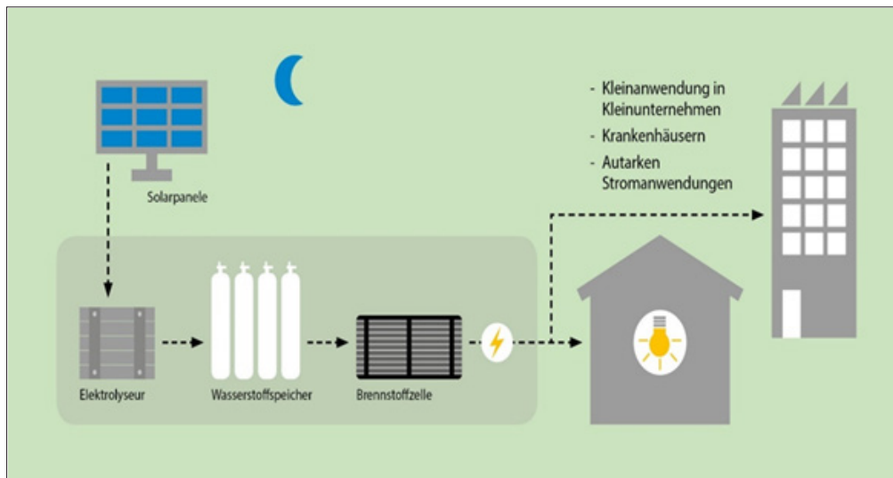
Figure 1: Concept of the Autark- Elys plant.
