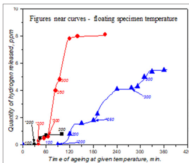
Figure 1: IPH degassing kinetics for irradiated steel ( 4,5 \times 10^{20} \text{ cm}^{-2} at 140 °C).
