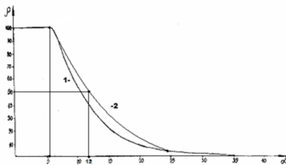
Figure 1: Nomogram of structural interaction degree dependence ( \rho ) on coefficient \alpha .
