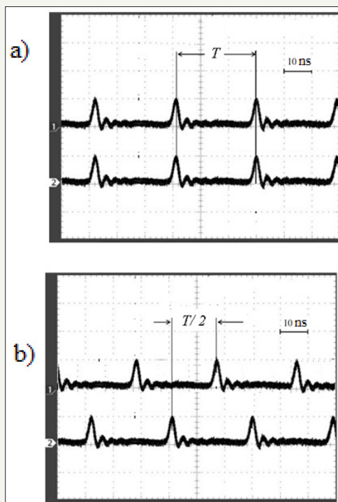
Figure 3: Oscillograms observed on the oscilloscope screen at a synchrotron radiation speed of light equal to (a) c and (b) 2c .
