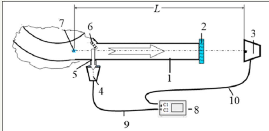
Figure 2: Proposed schematic of the measurements: (1) radiation output channel; (2) output window; (3) radiation detector of the measuring channel; (4) detector of the reference channel; (5) reference radiation output channel; (6) mirror of the reference channel output; (7) point of emission of an electron from a stationary orbit; (8) two-beam oscilloscope; (9) reference channel cable; (10) measuring channel cable.
