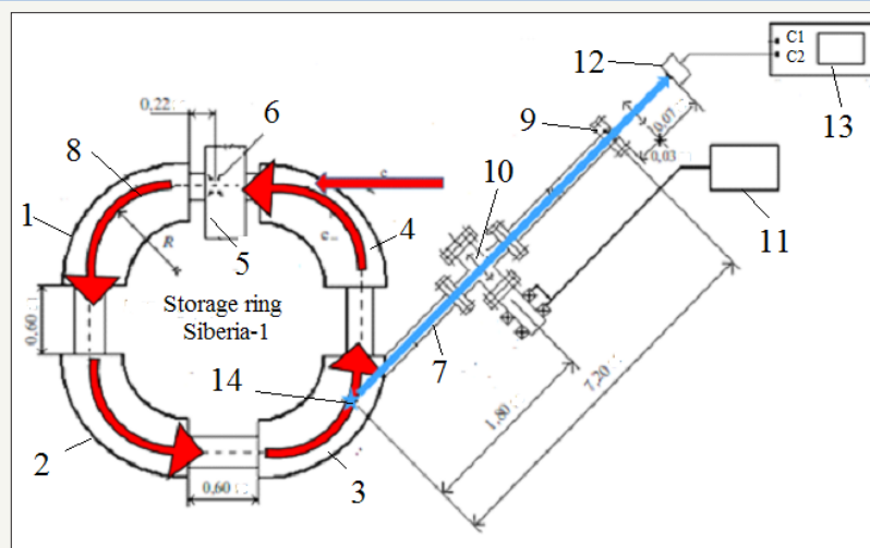
Figure 1: Schematic of the experiment: (1--4) rotary corner magnets; (5) resonator; (6) accelerating gap; (7) output channel of synchrotron radiation; (8) stationary orbit; (9) output window; (10) glass plate input/output system (IOS); (11) IOS control unit; (12) radiation detector; (13) oscilloscope; (14) point of emission. The distances are given in meters.
