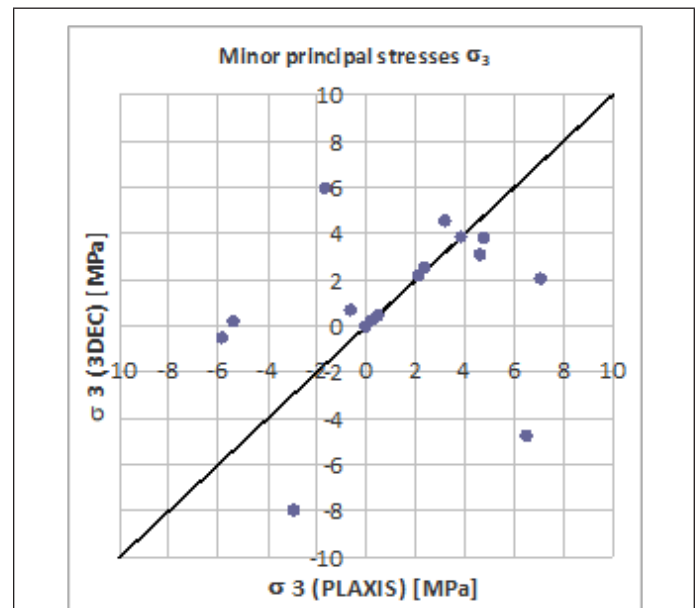
Figure 6: Minor principal stresses at the monitoring points.
