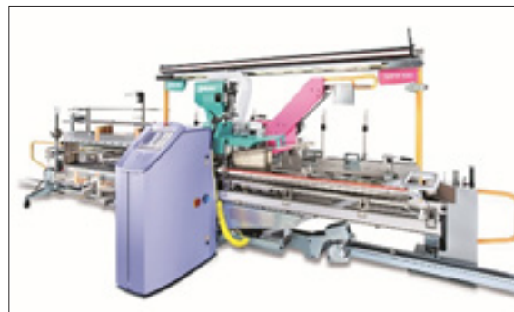
Figure 5: SAFIR S40 automatic drawing-in machine - Featuring Active Warp Control technology for yarn sorting.
