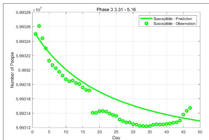
Figure 9: Result of curve fitting for the susceptible S(t) in Phase 3 (2020.3.31-2020.5.16).
