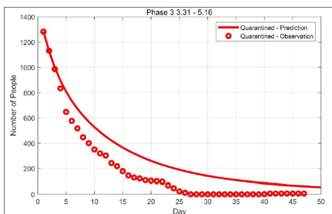
Figure 10: Result of curve fitting for the quarantined Q(t) in Phase 3 (2020.3.31-2020.5.16).
