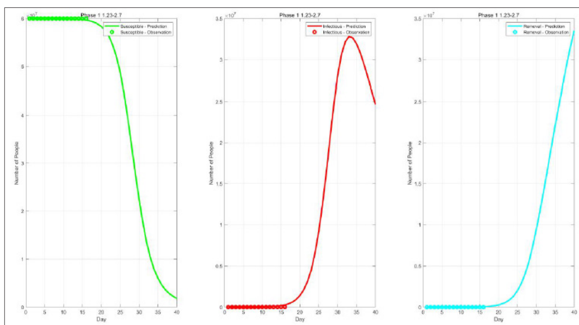
Figure 5: Result of curve fitting in Phase 1 (2020.1.23 - 2020.2.7).
