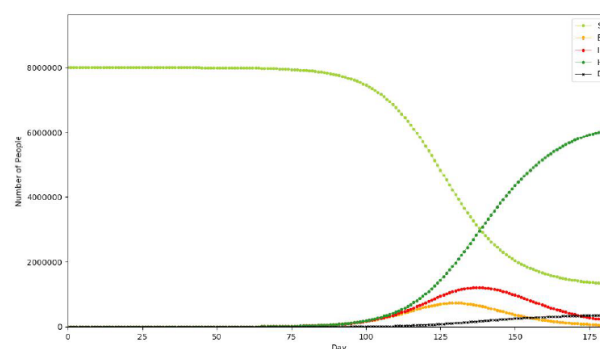
Figure 12: Result of SEIR simulation.
